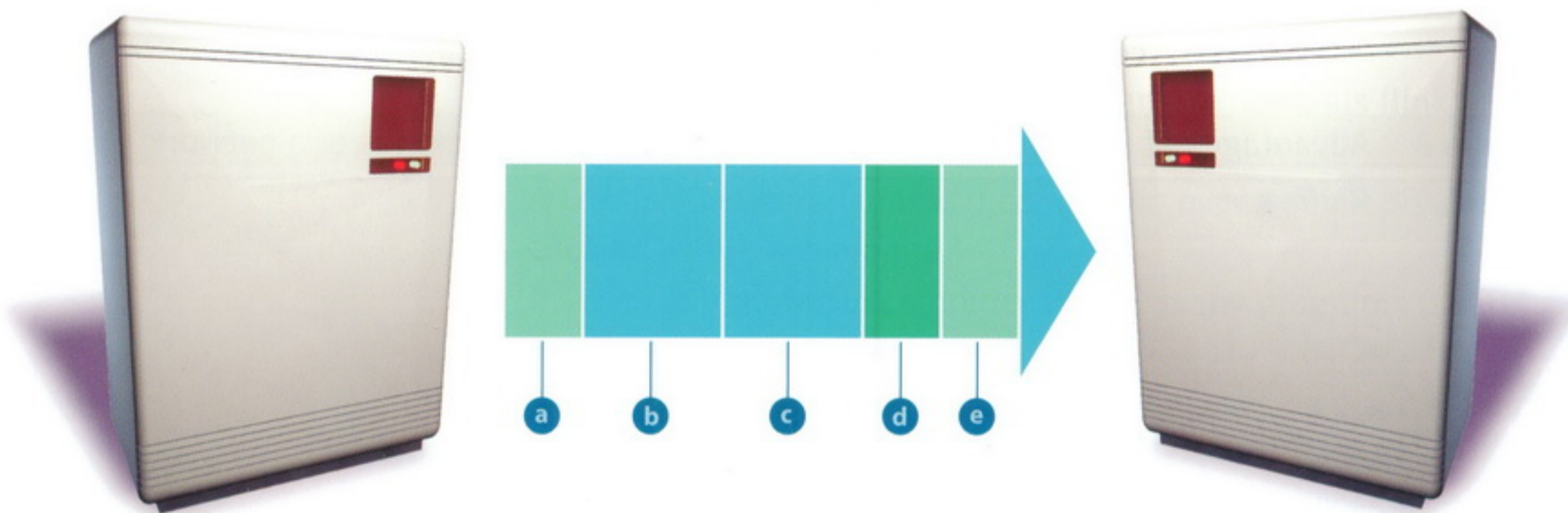
Fig 4 Synchronous transmission
