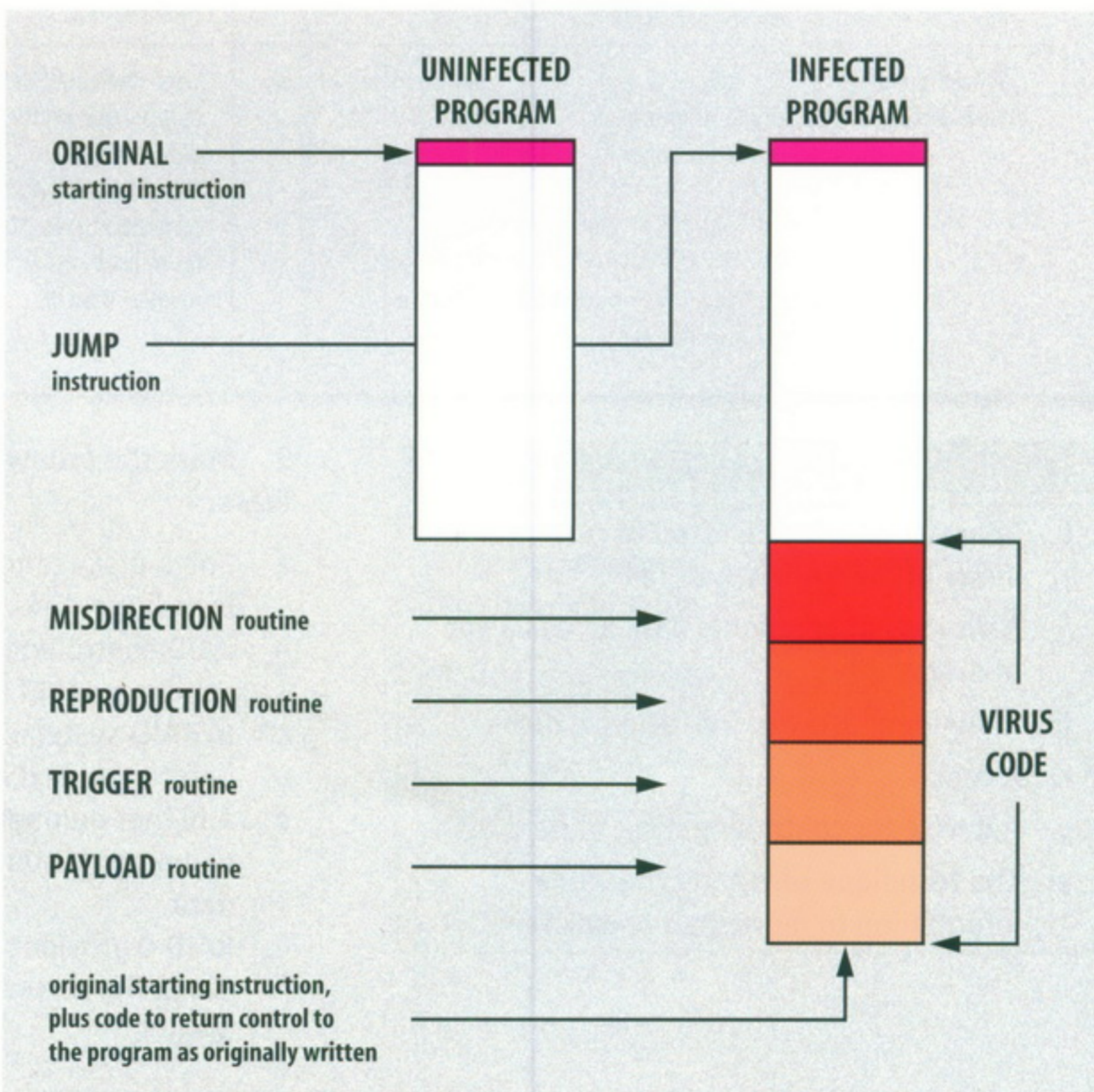
Fig 1 How a virus infects a program
