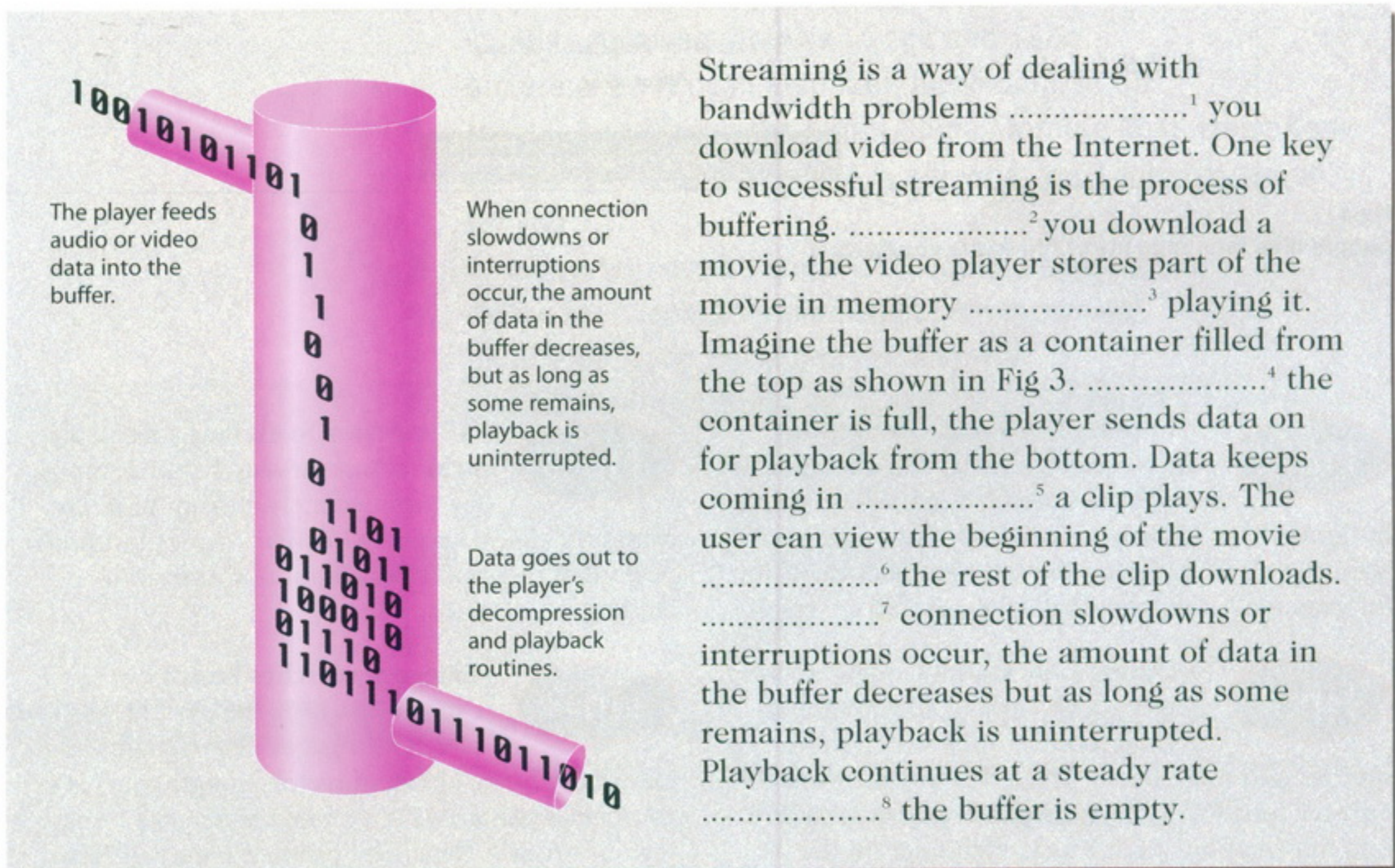
Fig 3 Video buffering
