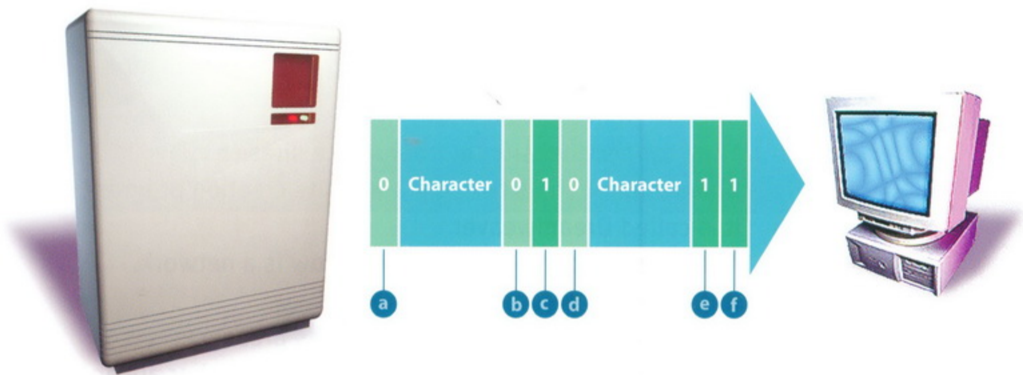
Fig 3 Asynchronous transmission
