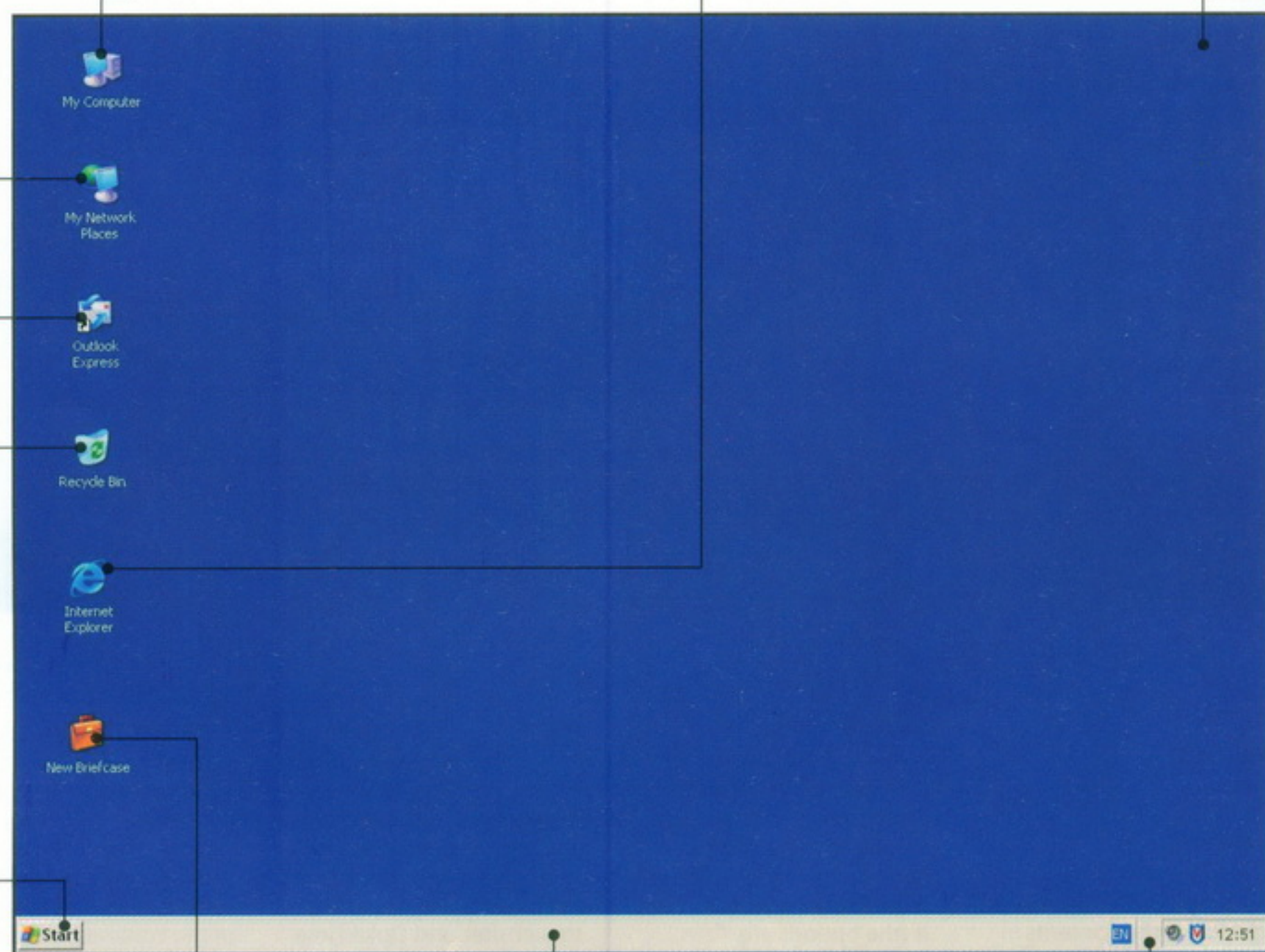
Fig 3 Windows desktop
